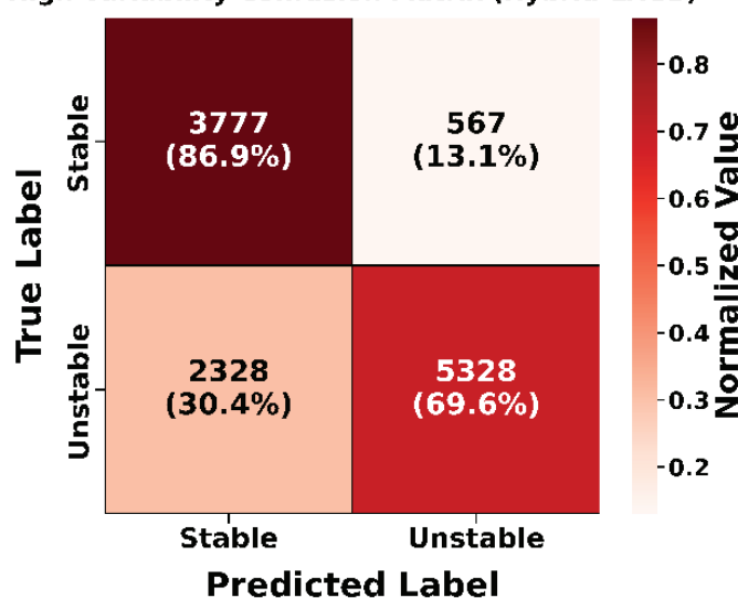
(c) Hybrid-LXGB
