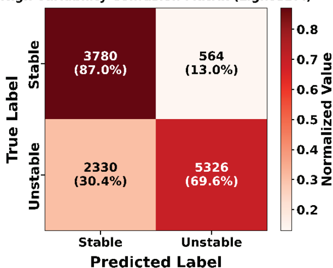
(a) LightGBM
