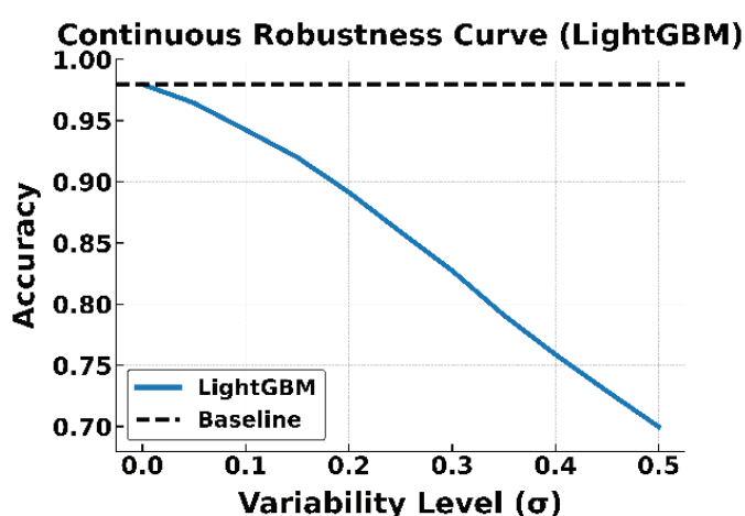
(a) LightGBM
