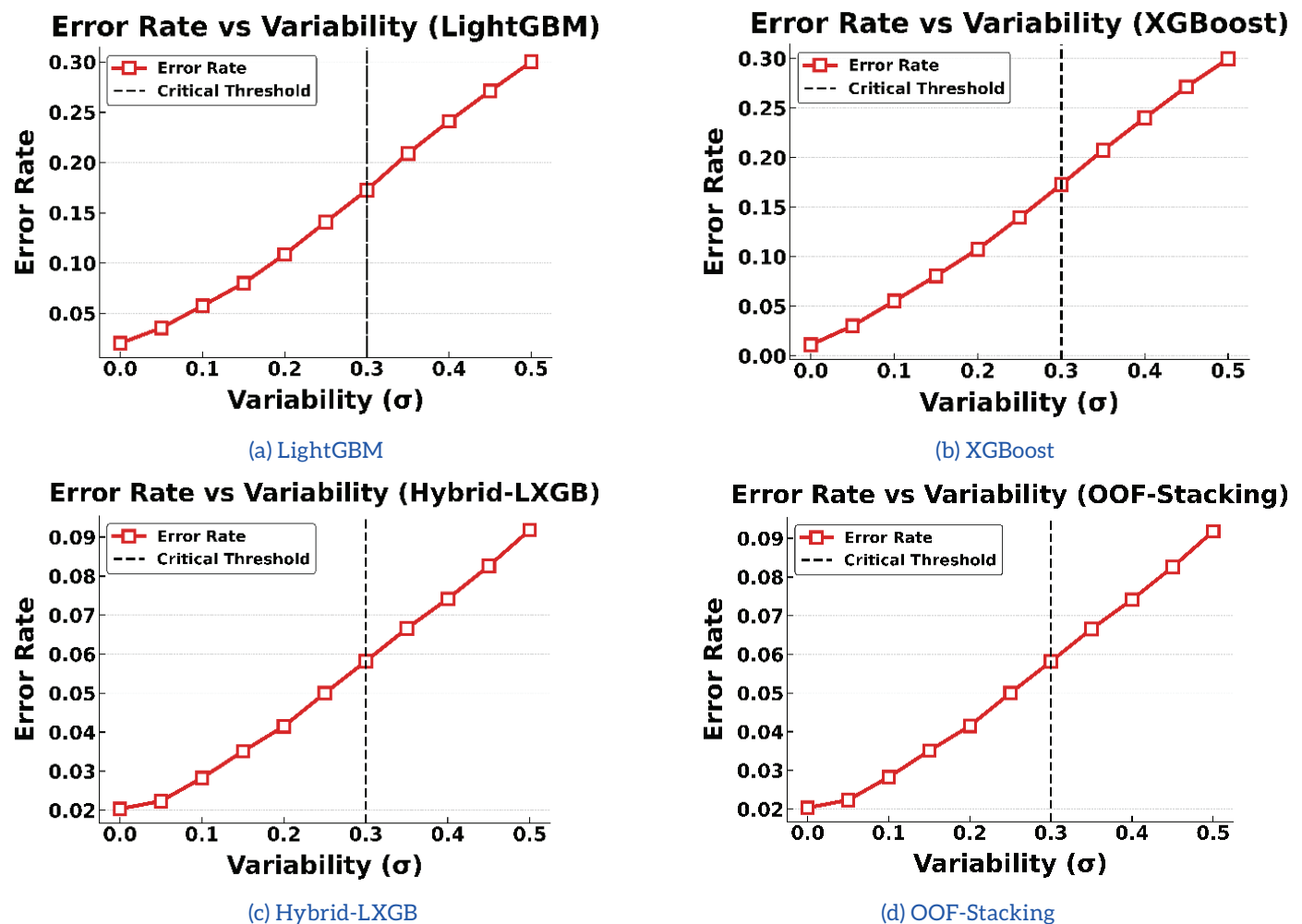
Figure 8: Continuous robustness curves showing accuracy variation with variability intensity ( \sigma ).
