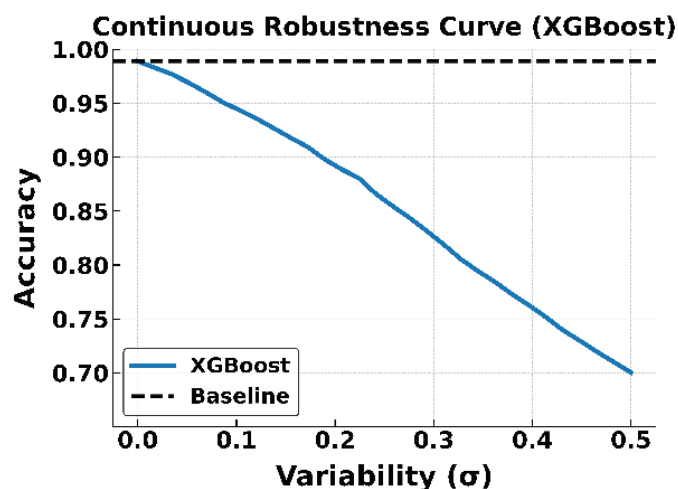
(b) XGBoost
