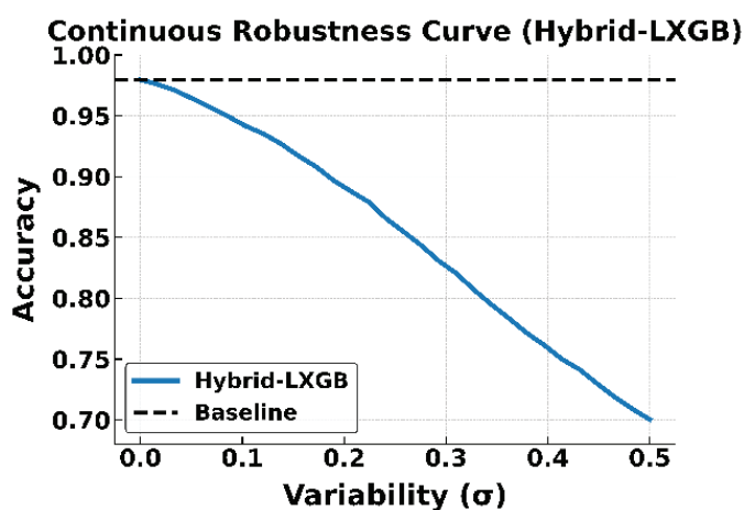
(c) Hybrid-LXGB
