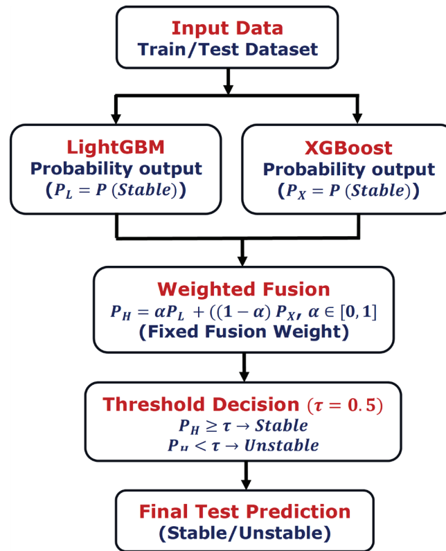
Figure 3: Hybrid-LXGB architecture using weighted fusion of LightGBM and XGBoost outputs.
