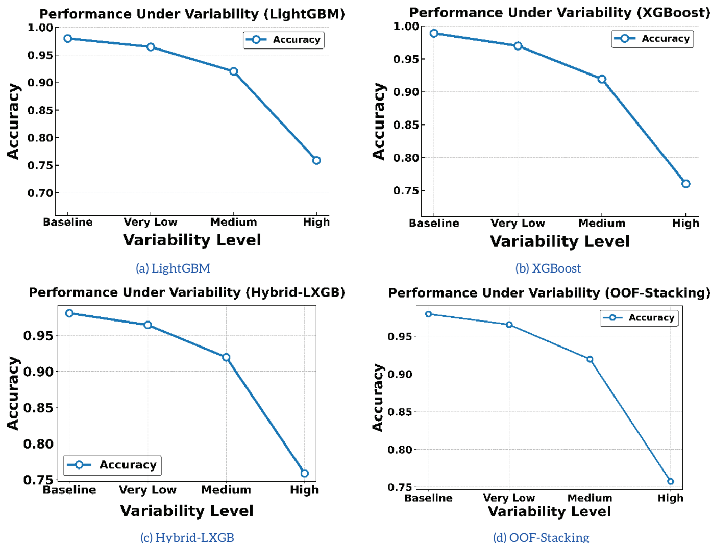
Figure 5: Accuracy comparison of all models under baseline and increasing variability conditions.
