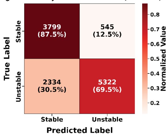
(b) XGBoost
