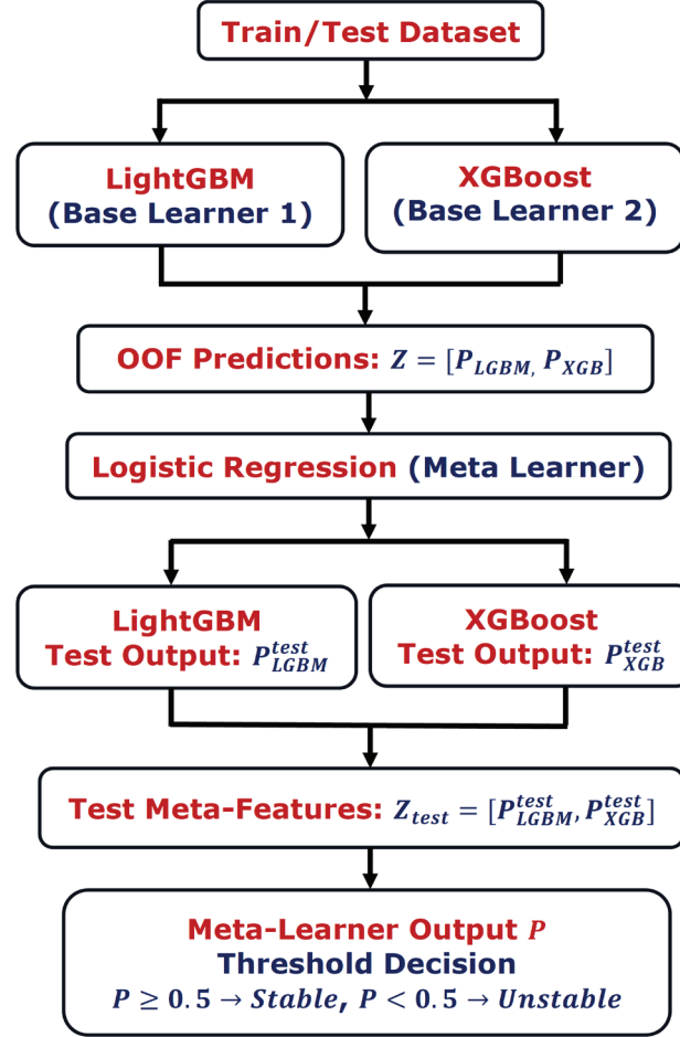
Figure 4: OOF-Stacking architecture using LightGBM and XGBoost base learners with logistic regression meta-learning.
