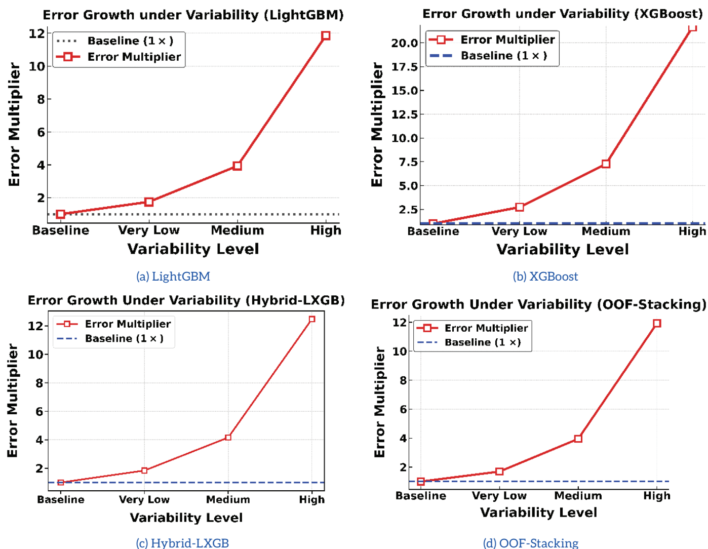
Figure 6: Comparison of accuracy degradation trends across models under varying disturbance levels.
