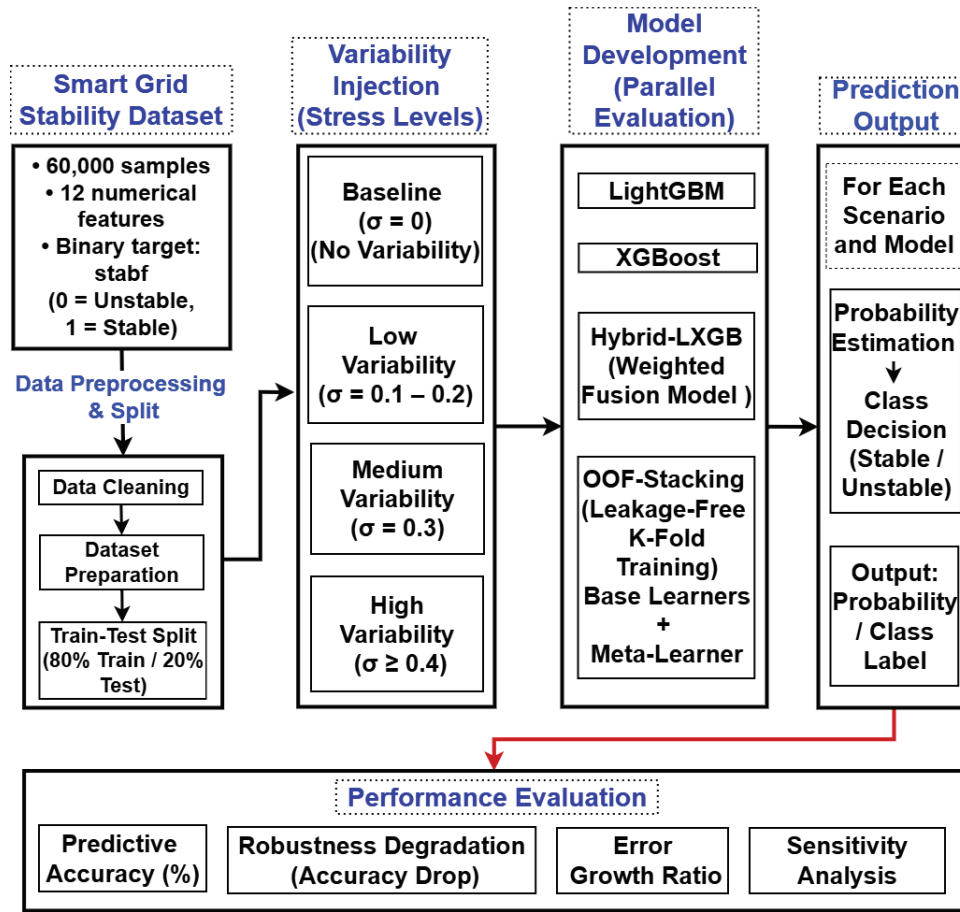
Figure 2: Overall comparative framework for robustness-oriented smart grid stability prediction.
