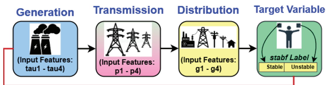
Figure 1: Structure of input feature categories and grid stability target variables.
