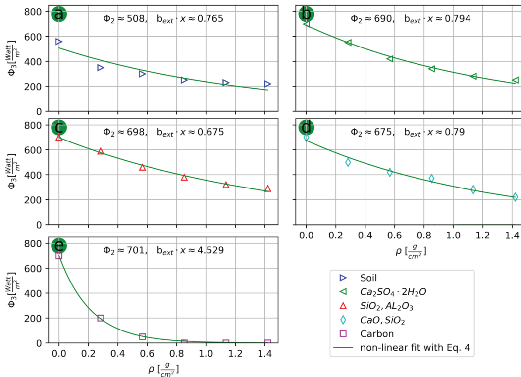
Fig.8. \Phi_3 - \rho Curves with their Fitting Curves to Find the Value of b_{\text{ext}} \cdot x
