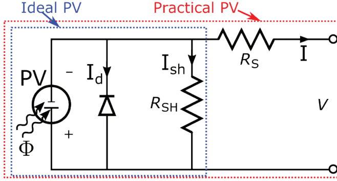
Fig.1. Solar Cell Internal Circuit
