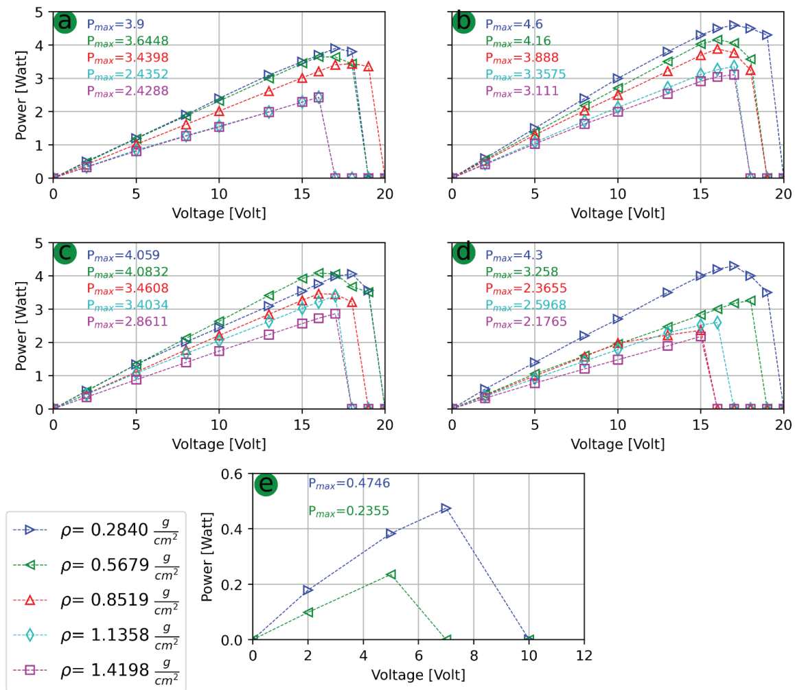
Fig.6. V-P Curves Characterization a: Soil, b: \text{Ca}_2\text{SO}_4 \cdot 2\text{H}_2\text{O} , c: \text{Al}_2\text{O}_3 , \text{SiO}_2 d: \text{CaO} , \text{SiO}_2 ,
