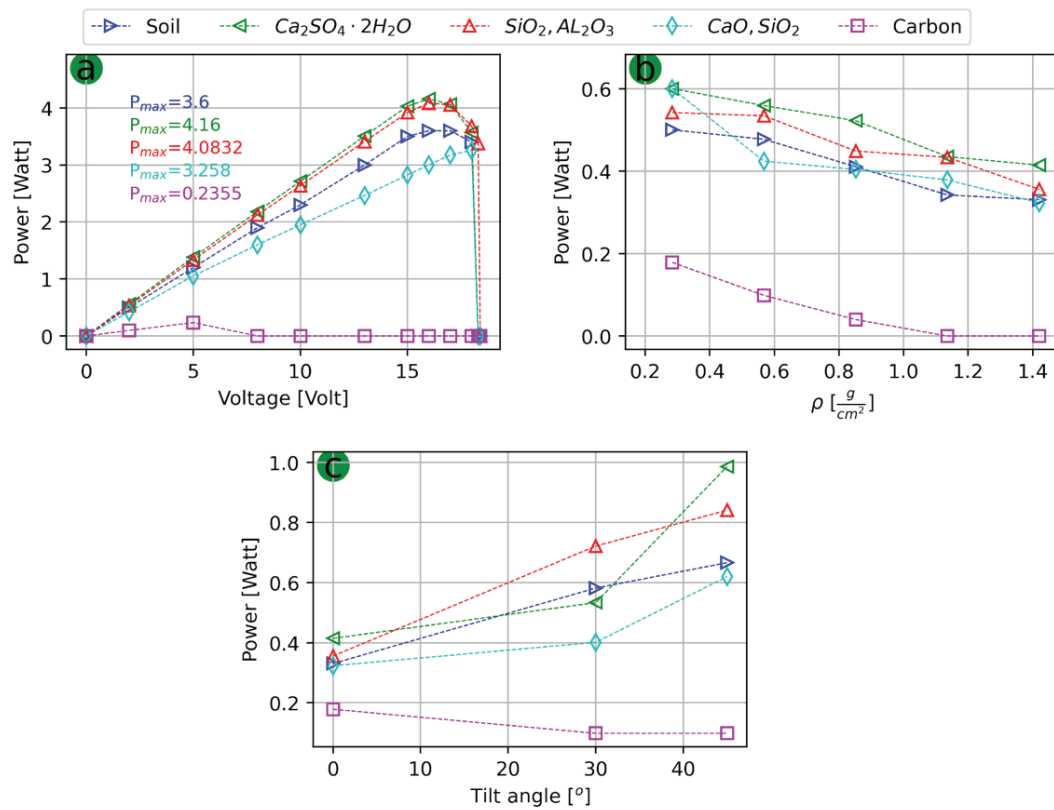
Fig.7. Curves of All Pollutants a: P - V curves, b: P - \rho curves c: P - tilt angle curve
