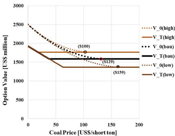
Fig .3. Option values at various electricity prices from renewable sources
