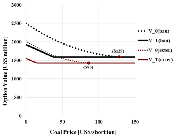
Fig .5. Option values with externality cost for using coal
