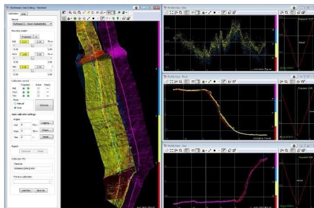
Figure 3: Displays patch test Calibration and results, PDS 2000.
