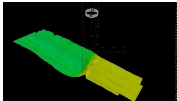
Figure 5: The processing of Hydrographic survey data, PDS 2000.
