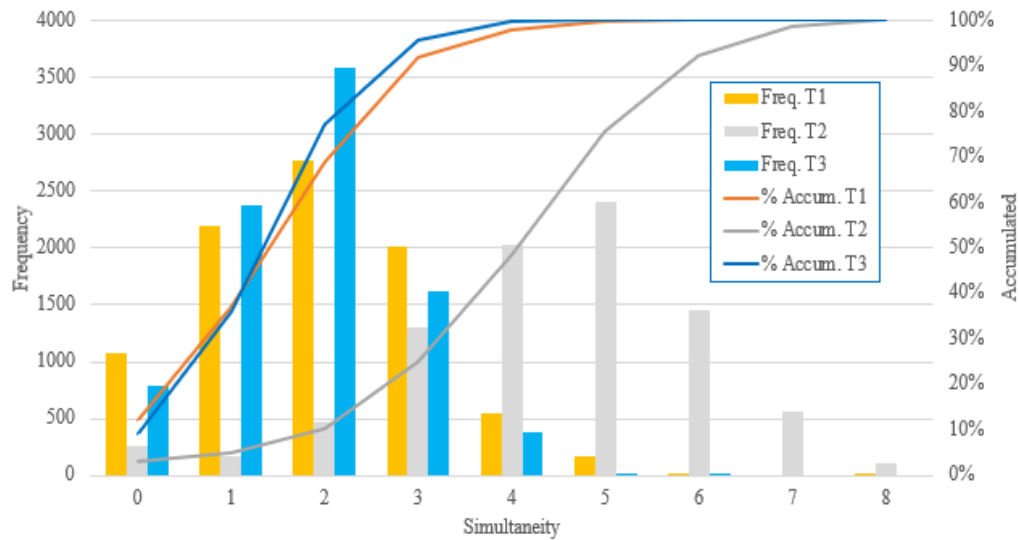
Figure 5: Simultaneity at Container Ship Terminals. Source: Siport21.
