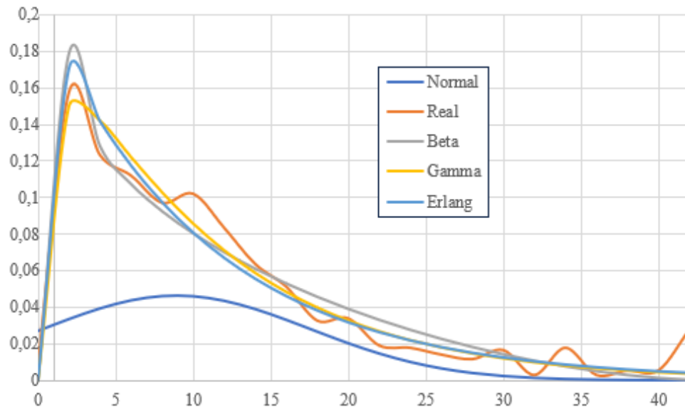
Figure 8: Search of the Closest Fit Distribution. Source: Siport21.
