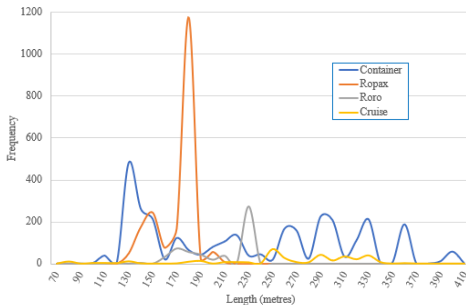
Figure 1: Vessel Size Depending on Cargo. Source: Siport21.
