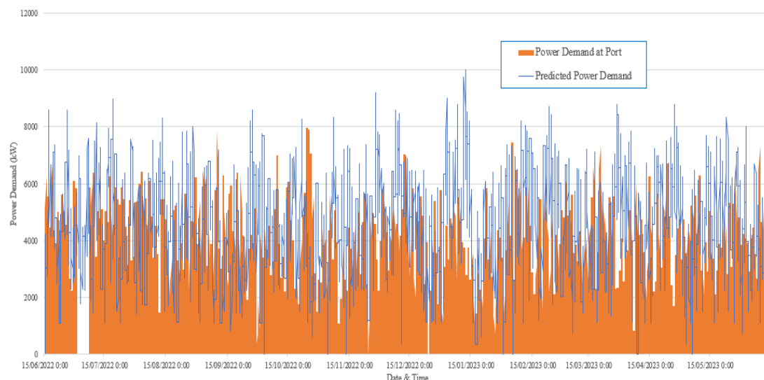
Figure 9: Power Demand Forecast at Container Terminal Based on Historical Data. Source: Siport21.
