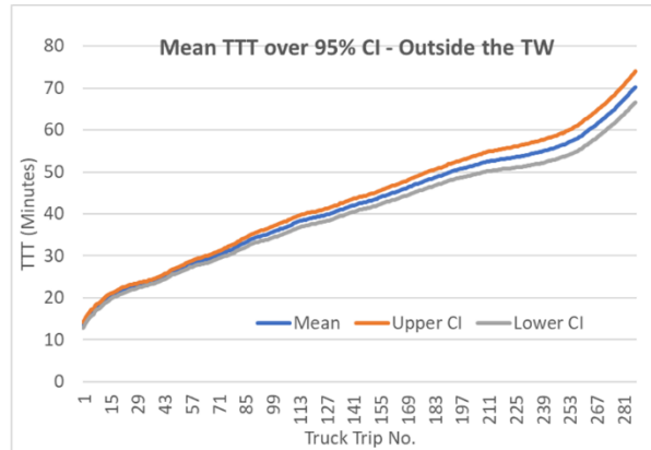
Figure 11: Plot of cumulative mean TTT over 95% CI for arrivals outside TW
