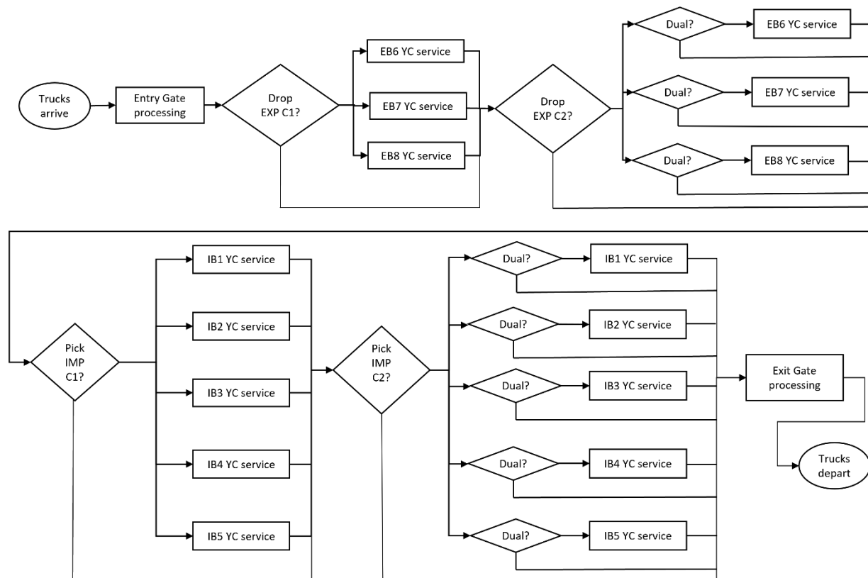
Figure 3: Process flow of container drop-off and pickup operations.
