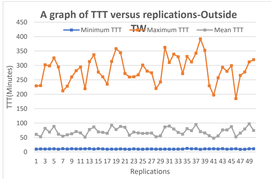
Figure 7: Line Plot of Average Truck Turnaround Times (Outside the TW).
