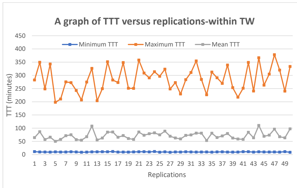
Figure 6: Line Plot of Average Truck Turnaround Times (Within the TW).
