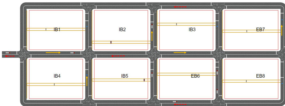
Figure 2: 2-D CT simulation model (yard area).
