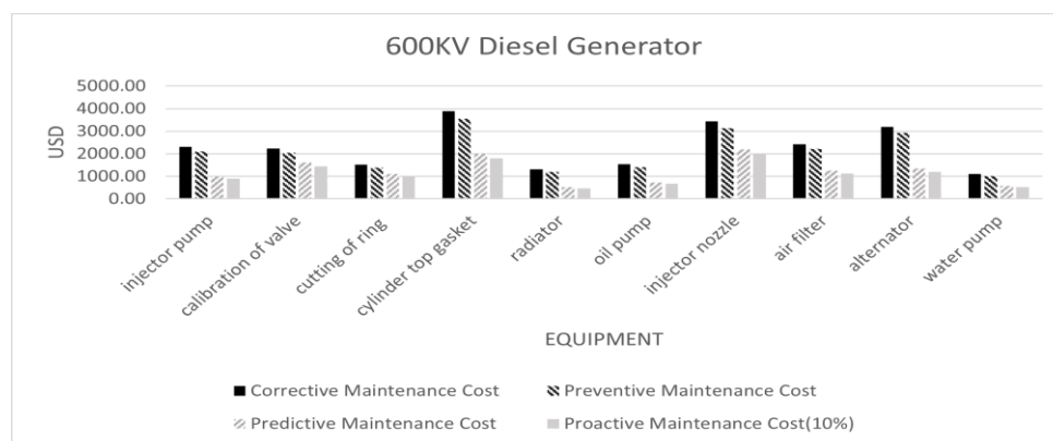
Figure 3: Cost of Different Maintenance Strategies for 600 kV Diesel Generator
