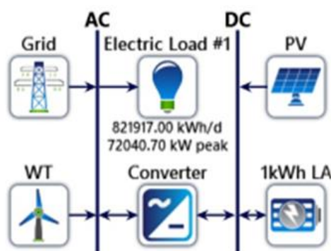
Figure 5: Schematic Diagram of the Relations Between Grid and Renewable Application.
