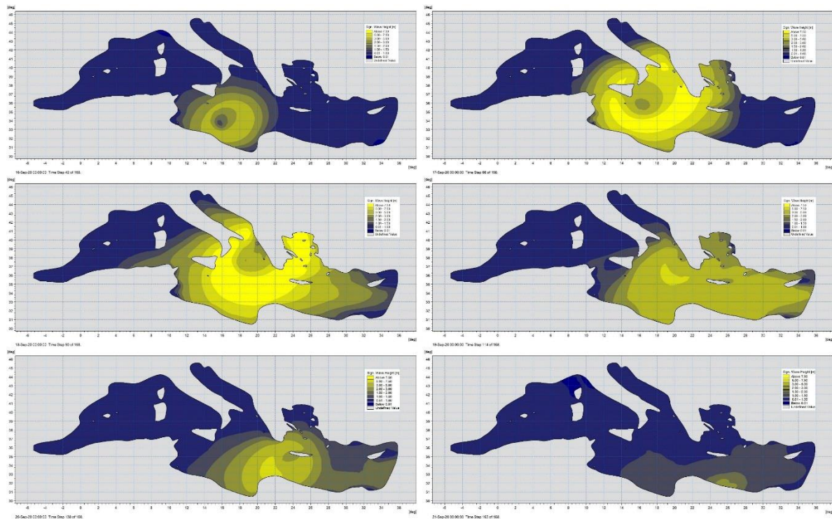
Figure 7: Resulted oceanographical wave height during Medicane lanos from September 16 to September 21, 2020, with a time step of 24 hours.
