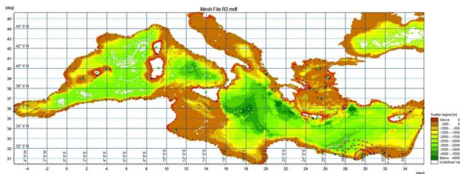
Figure 6: Generated mesh file for the numerical modelling with projection of WGS-84/EPSSG 4326.
