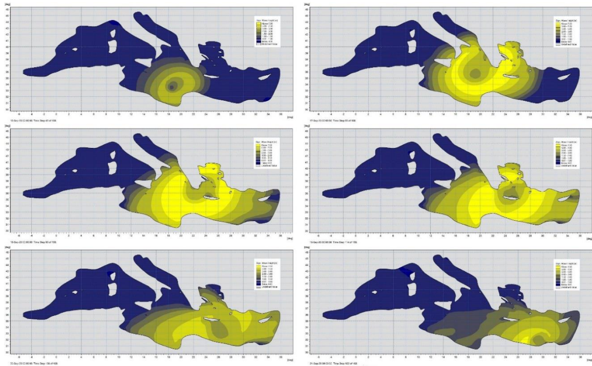
Figure 11: Resulted expected oceanographical wave height during 100-year return period Medicanne from September 16 to September 21, with a time step of 24 hours.
