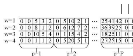
Figure 2: The schematic of the coding of a chromosome
