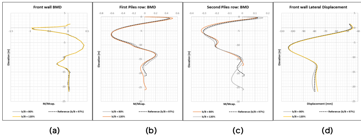
Figure 12: Impact of adjusting bearing level of piles when sand fill is backfill: (a) Front wall BMD, (b) 1st piles row BMD, (c) 2nd piles row BMD, (d) Lateral displacement
