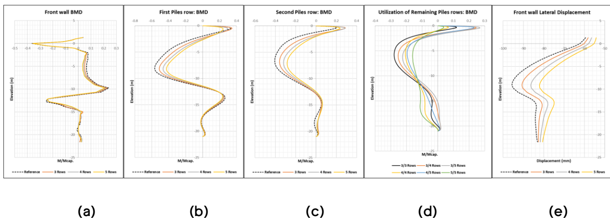
Figure 8: Impact of adjusting number of piles when OC clay is used as backfill soil: (a) Front wall BMD, (b) 1 st piles row BMD, (c) 2 nd piles row BMD, (d) utilization of the remaining piles, (e) system displacement
