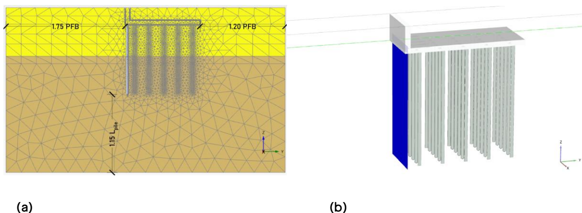
Figure 2: Numerical model: (a) Adopted meshing configuration, (b) perspective view of the model components
