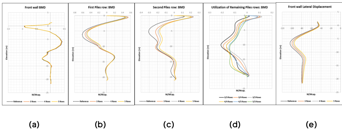
Figure 7: Impact of adjusting number of piles when sand fill is used as backfill soil: (a) Front wall BMD, (b) 1 st piles row BMD, (c) 2 nd piles row BMD, (d) utilization of the remaining piles, (e) system displacement
