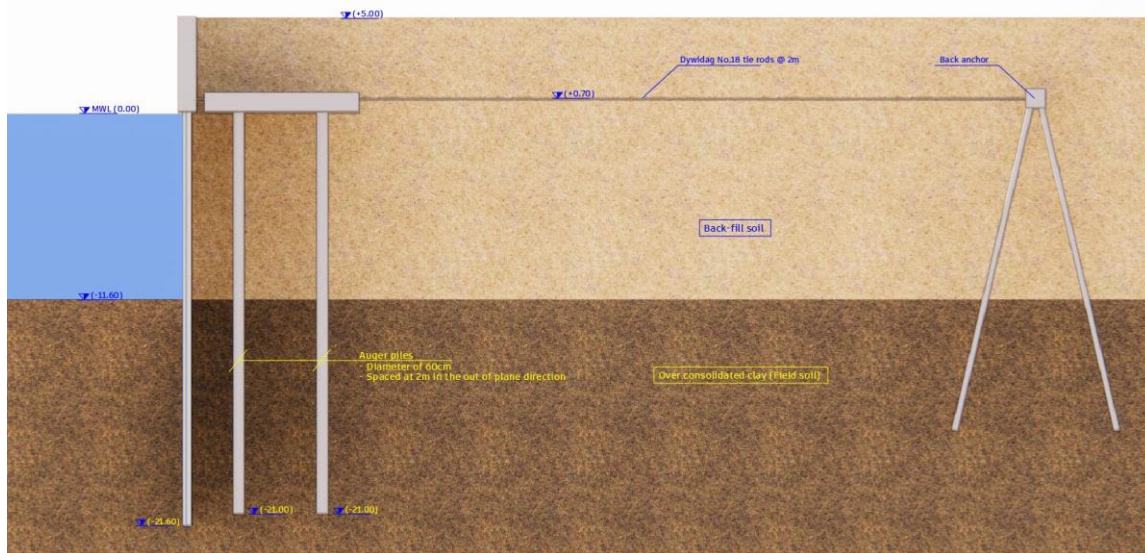
Figure 4: Typical cross-section of the basic reference models
