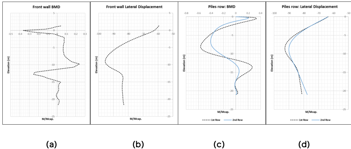
Figure 6: Straining actions of reference model 02: (a) Front wall BMD, (b) Front wall deflection, (c) Piles BMD, (d) Piles deflection
