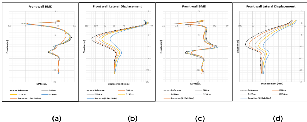
Figure 9: Impact of adjusting stiffness of piles: (a) Front wall BMD when sand fill is backfill, (b) lateral displacement when sand fill is backfill, (c) Front wall BMD when OC clay is backfill, (d) Lateral displacement when OC clay is backfill
