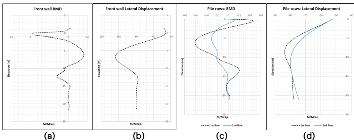
Figure 5: Straining actions of reference model 01: (a) Front wall BMD, (b) Front wall deflection, (c) Piles BMD, (d) Piles deflection
