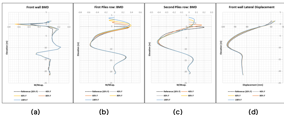
Figure 15: Impact of adjusting platform level when OC clay is backfill: (a) Front wall BMD, (b) 1st piles row BMD, (c) 2nd piles row BMD, (d) Lateral displacement
