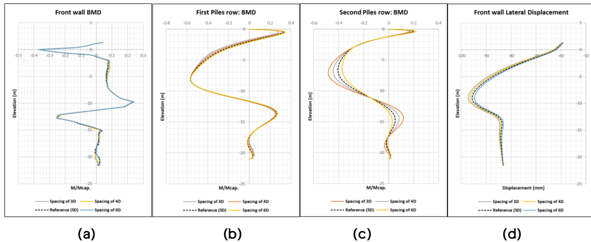
Figure 11: Impact of adjusting spacing of piles when OC clay is backfill: (a) Front wall BMD, (b) 1st piles row BMD, (c) 2nd piles row BMD, (d) Lateral displacement
