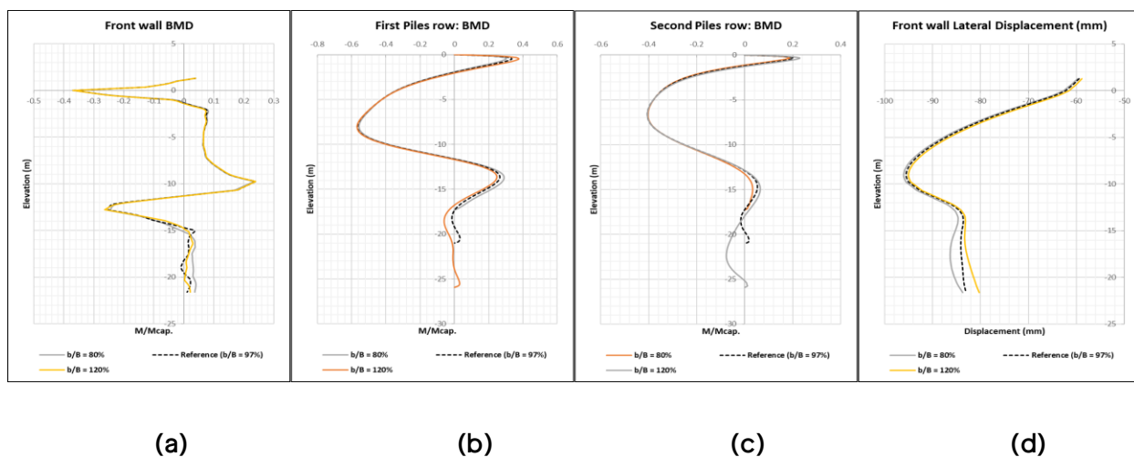
Figure 13: Impact of adjusting bearing level of piles when OC clay is backfill: (a) Front wall BMD, (b) 1st piles row BMD, (c) 2nd piles row BMD, (d) Lateral displacement
