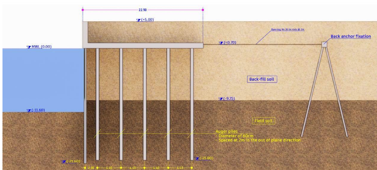
Figure 1: Cross-section of the measured quay wall
