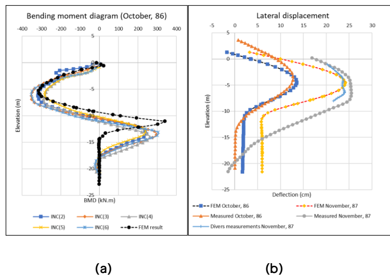
Figure 3: Front wall verification results: (a) Bening moments, (b) Lateral displacements
