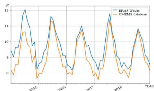
Figure 3: Comparison between shows time series of scatter index of H_s for CMEMS and ERA5 results
