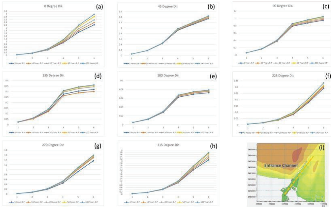
Figure 8 : Analyzed H_s Values for Entrance Channel Line for Different Direction and Various Return Periods of (a) 0^\circ (b) 45^\circ (c) 90^\circ (d) 135^\circ (e) 180^\circ (f) 225^\circ (g) 270^\circ (h) 315^\circ (i) Plan View for Entrance Channel Line
