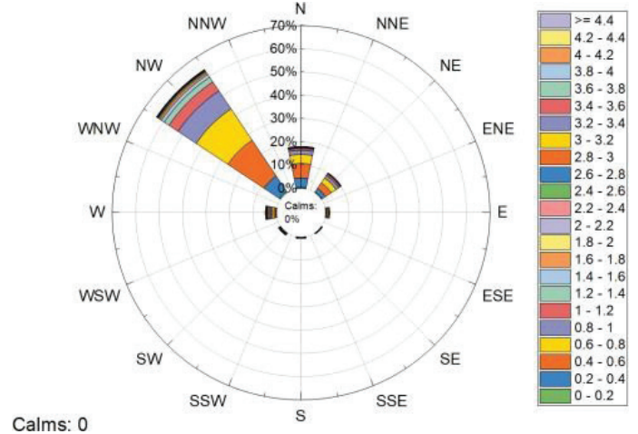
Figure 4: Wave Rose for Different Directions in front of Suez Canal, Port Said
