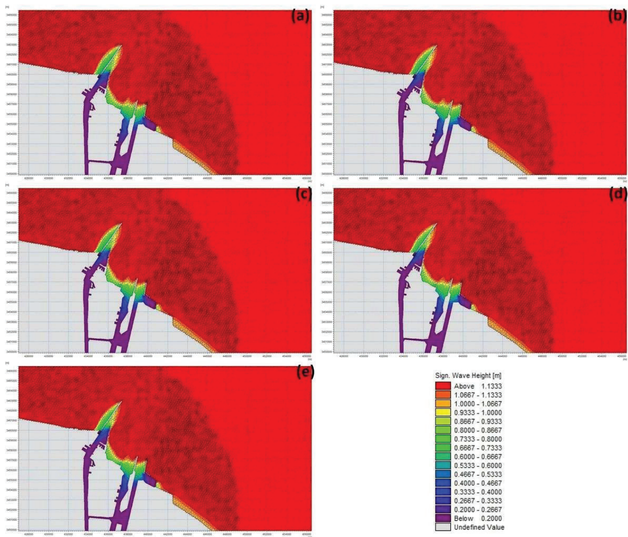
Figure 7 : H_s values at the Suez Canal zone for 45^\circ direction for different return period (a) 5 years return period (b) 10 years return period (c) 20 years return period (d) 50 years return period (e) 100 years return period.
