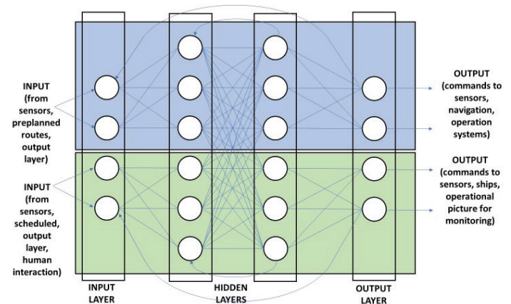
Figure 2: Proposed architecture for the recurrent neural network.
