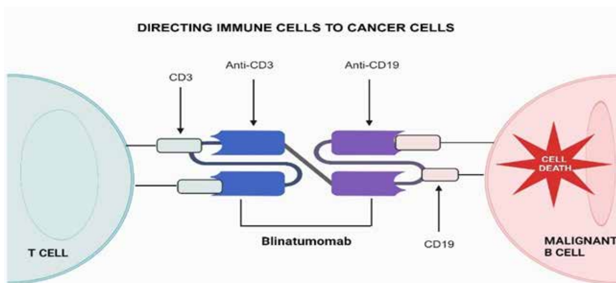
Figure 2 The mechanism of action for blinatumomab, the first-in-class BiTE, involves one arm binding to CD3 and the other to CD19. This interaction activates unstimulated T cells, initiating their attack on CD19+ cells.
