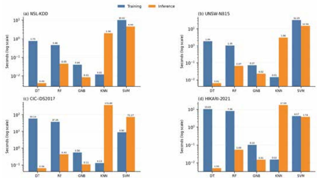
Figure 8: Training and inference time, ML models, all features, CPU only: (a) NSL-KDD; (b) UNSW-NB15; (c) CIC-IDS2017; (d) HIKARI-2021.
