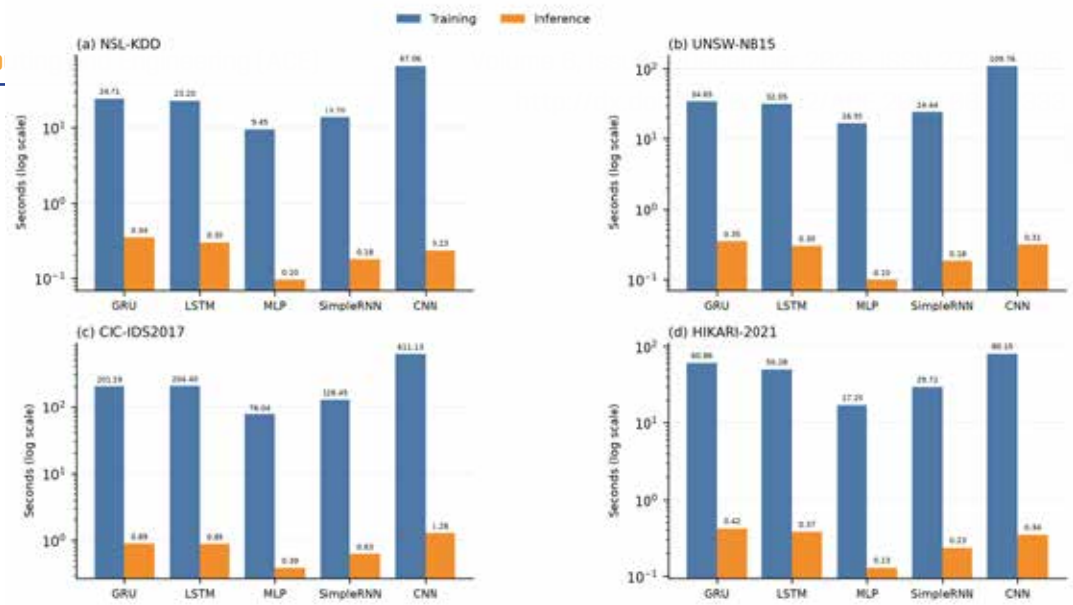
Figure 9: Training and inference time, DL models, all features, CPU only: (a) NSL-KDD; (b) UNSW-NB15; (c) CIC-IDS2017; (d) HIKARI-2021.
