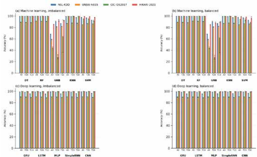
Figure 2: Accuracy across datasets: (a) ML models, imbalanced; (b) ML models, balanced; (c) DL models, imbalanced; (d) DL models, balanced.
