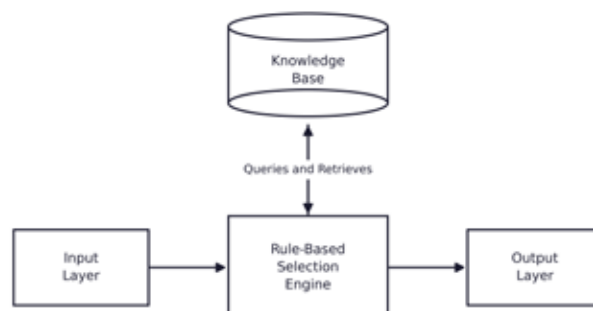
Figure 13: Components of IDS-ReComm: Input Layer, Rule-Based Selection Engine, Knowledge Base, and Output Layer.
