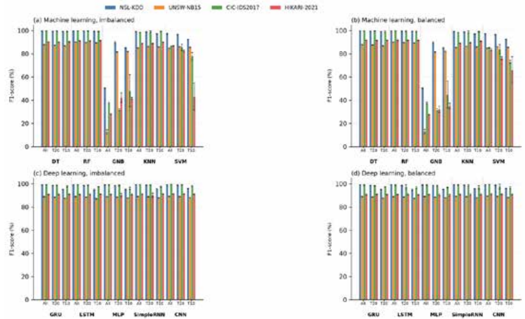
Figure 5: F1-score across datasets: (a) ML, imbalanced; (b) ML, balanced; (c) DL, imbalanced; (d) DL, balanced.
