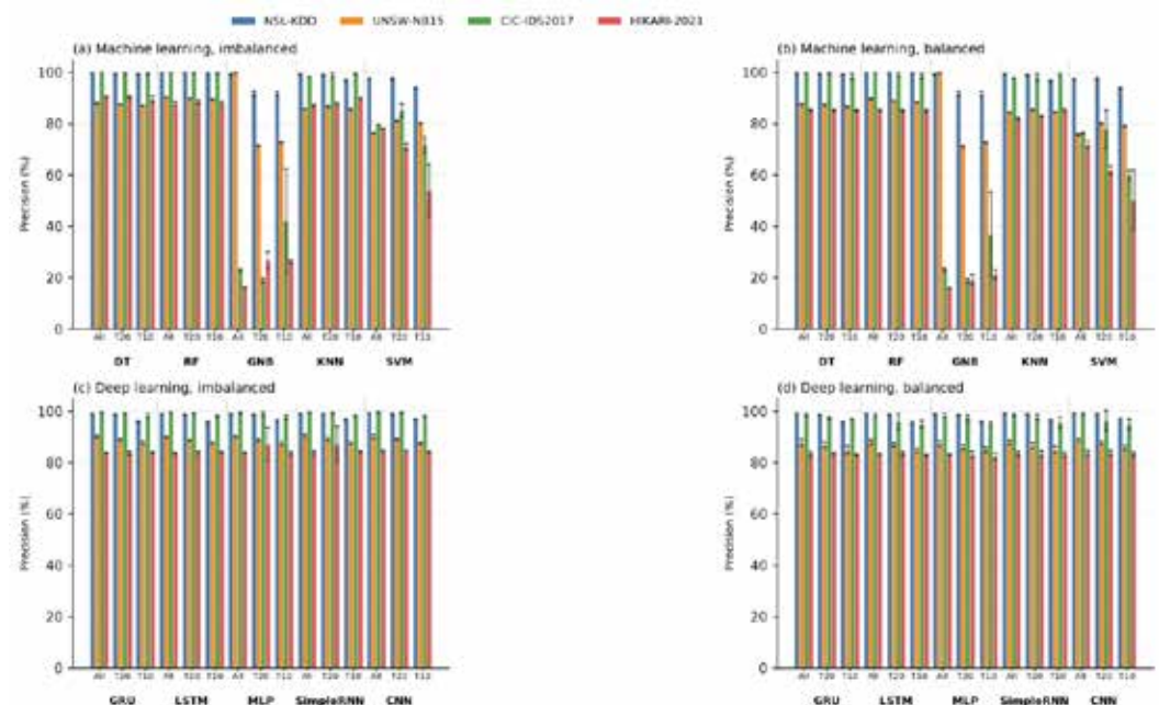
Figure 4: Precision across datasets: (a) ML, imbalanced; (b) ML, balanced; (c) DL, imbalanced; (d) DL, balanced.
