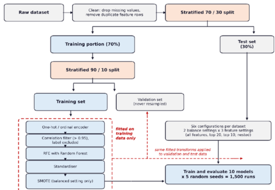
Figure 1: Experimental pipeline. Every transform is fitted on the training split alone and applied to validation and test data.
