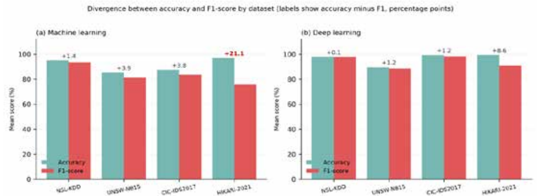
Figure 10: Divergence between accuracy and F1-score by dataset. Labels show accuracy minus F1-score in percentage points.
