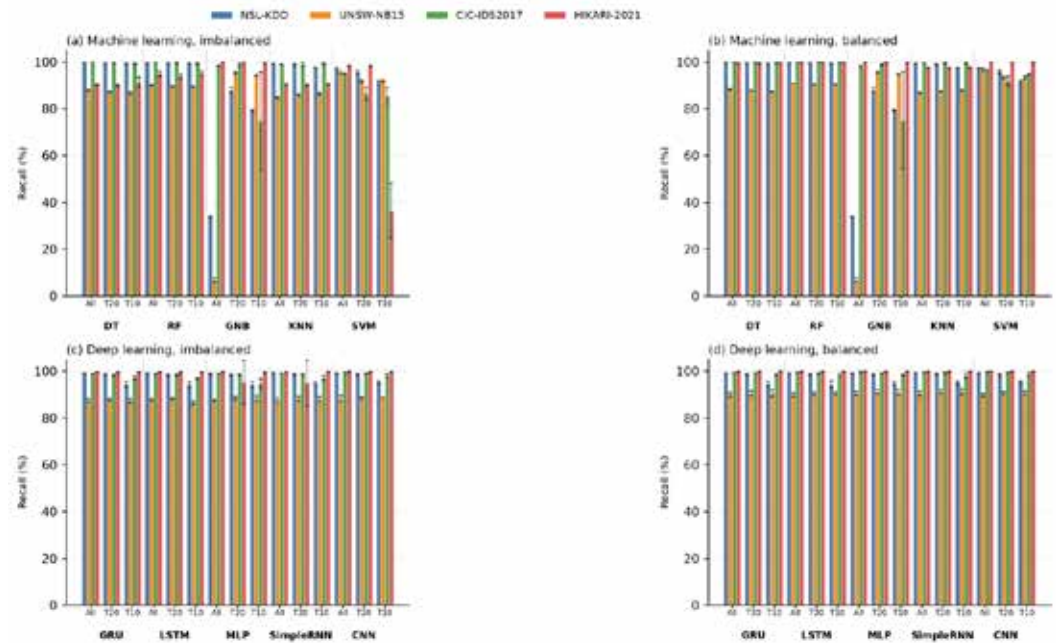
Figure 3: Recall across datasets: (a) ML, imbalanced; (b) ML, balanced; (c) DL, imbalanced; (d) DL, balanced.
