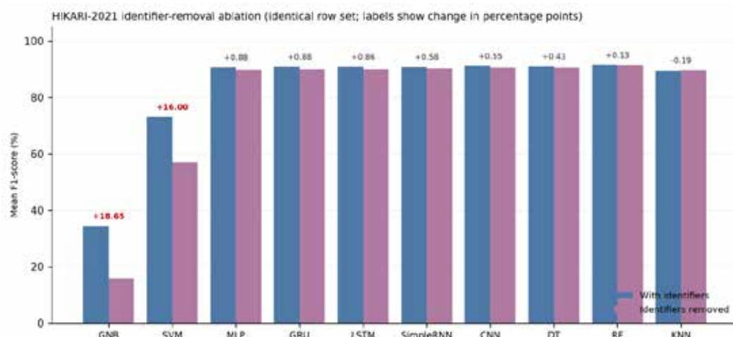
Figure 11: HIKARI-2021 identifier-removal ablation on an identical row set. Labels show the change in mean F1-score in percentage points.
