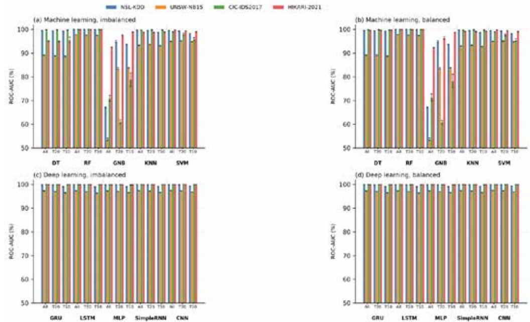
Figure 6: ROC-AUC across datasets: (a) ML, imbalanced; (b) ML, balanced; (c) DL, imbalanced; (d) DL, balanced.
